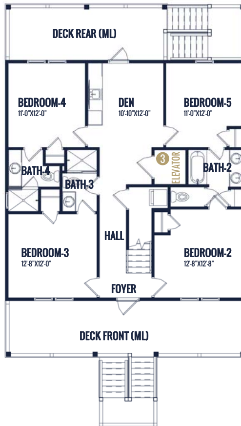
MAIN LEVEL
